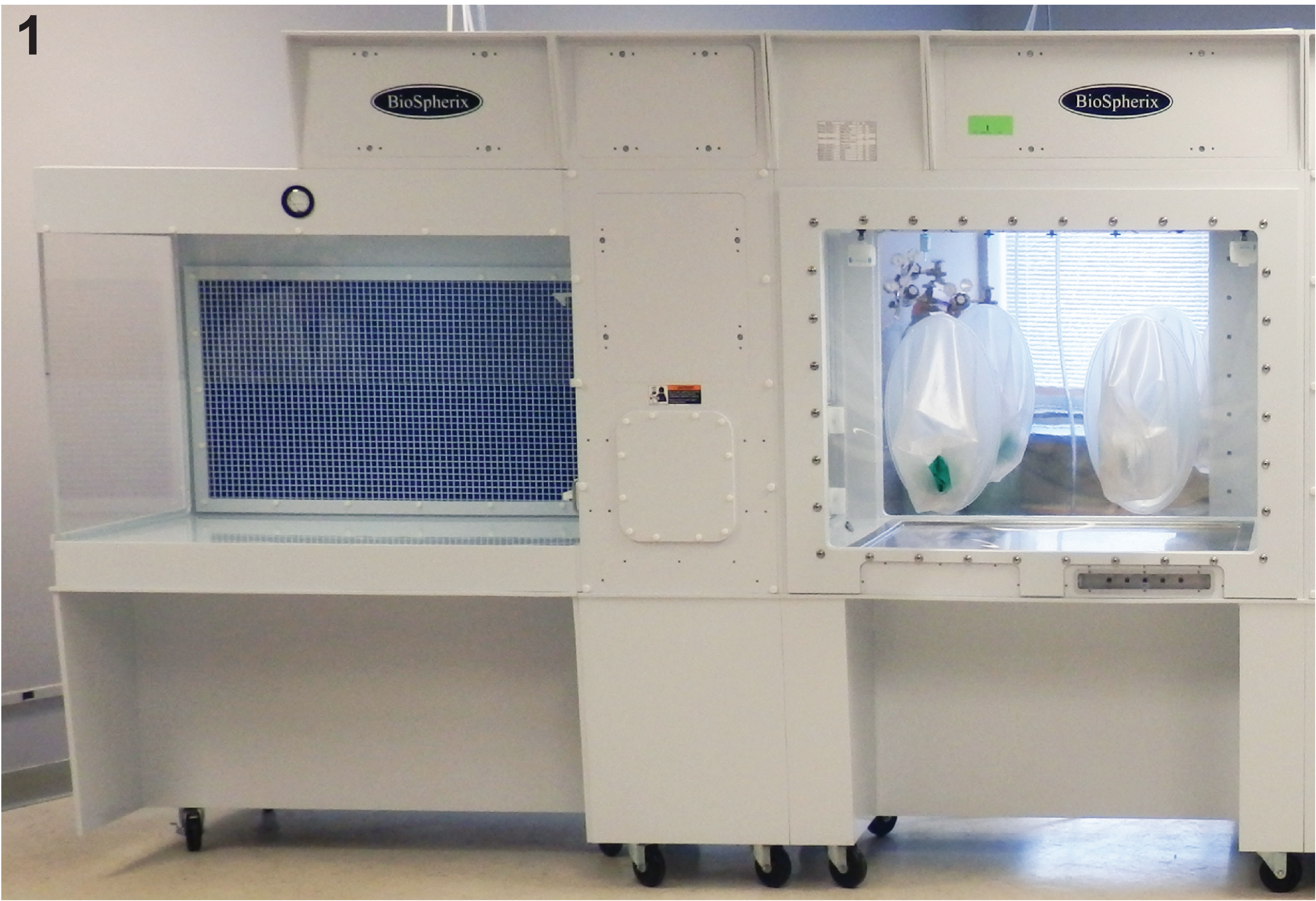
Figure 1. Experimental Set-Up
